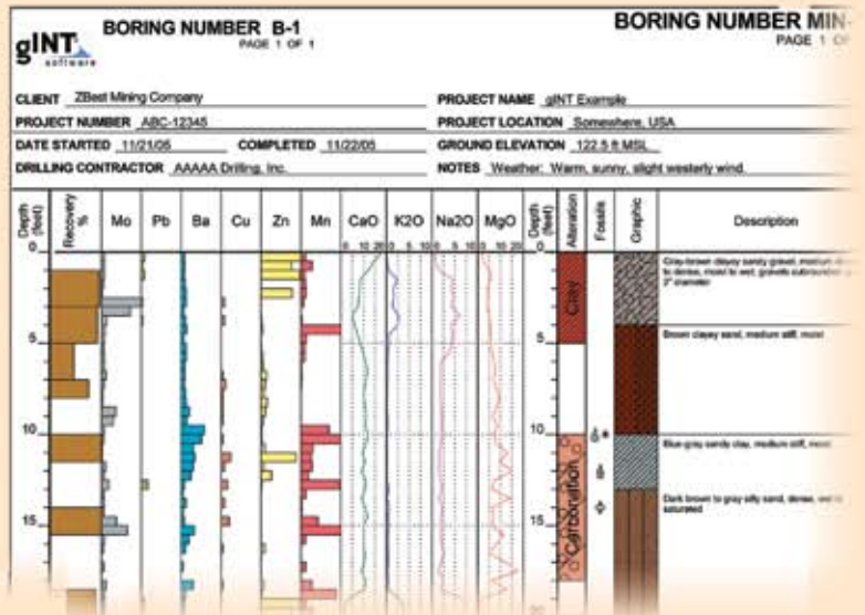
Mining Log
