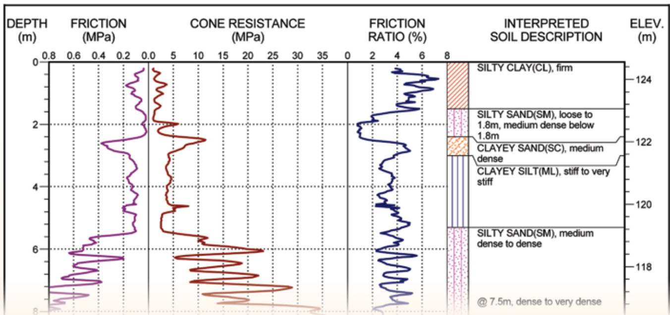
Cone Penetrometer Test Log
