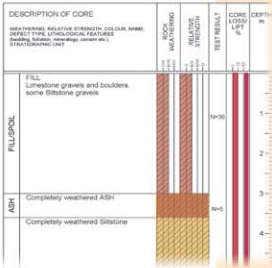
Rock Log
