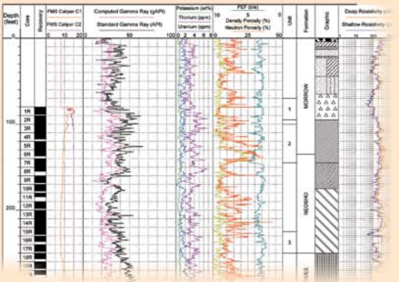
Geophysical Log
